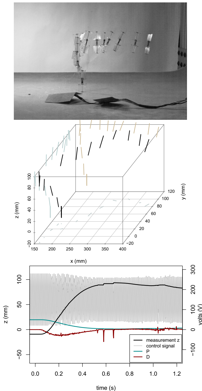
Fig. 8. Composite image from frames of a high speed video of altitude control of flapping microrobotic bee commanded to an altitude of 100 mm (top). Here the RoboBee accelerates vertically until reaching an altitude setpoint, then begins to drift laterally. A 3D plot of the RoboBee's trajectory (shown with its shadow) shows lateral drift in both the x and y axis which could be due to a combination of inherent torque bias and lateral motions during stabilization of \theta . Each point in the 3D plot is 50 ms apart (middle). During the trial, we recorded the altitude measured by visual tracking (bottom, left axis), the P and D amplitude control commands, and piezoelectric actuator voltage during this trial run (bottom, right axis).
