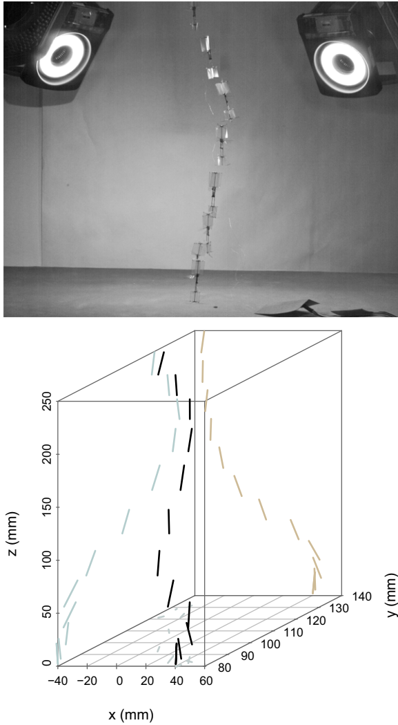
Fig. 7. Composite image from frames of a high speed video of a stable vertical takeoff by the damper-stabilized RoboBee with the corresponding 3D plot of its trajectory. Shutter speed was 1/500 s and frame interval is 0.1 s (top). A 3D plot of its trajectory (black) shown with its projections on the xy (grey), xz (beige) and yz (blue) plane (bottom). Each point in the 3D plot is 50 ms apart.
