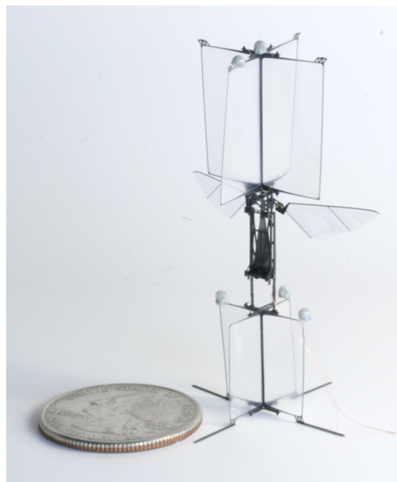
Fig. 1. Image of the RoboBee with 20 mm square top damper and 15 mm square bottom damper.
