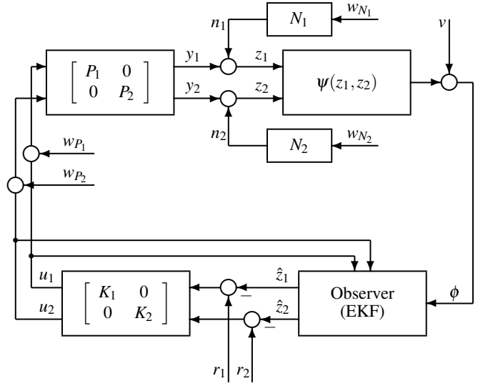
Fig. 6. Signals-and-systems block diagram idealization of the optical system with proposed control scheme.
