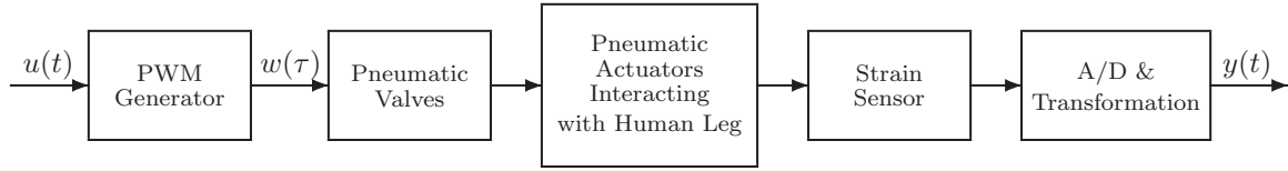
Figure 10. Upper-level physical description of the system from an input–output perspective, according the definitions of u(t) and y(t) . Note that y(t) is a physical variable (angular position), whereas u(t) is not a physical entity but a mathematical tool used for controller design.
